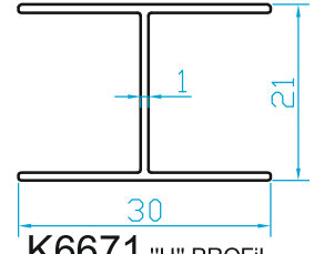
K6671 'H' PROFİL (0.215 Kg/m)
