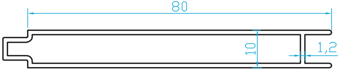
K517 TAHTA LAMBRI (1 mm) (0.600 Kg/m)
