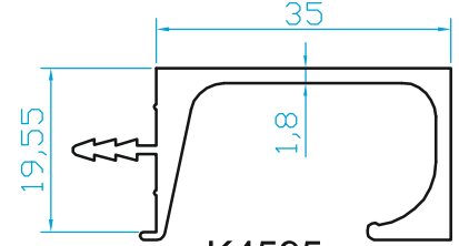
K4595 MOBİLYA PROFİLİ 0.540 Kg/m
