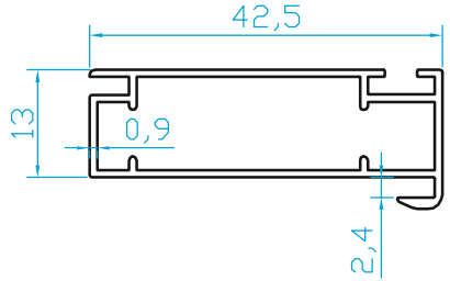
K6875 MOBİLYA PROFİLİ (0.340 Kg/m)
