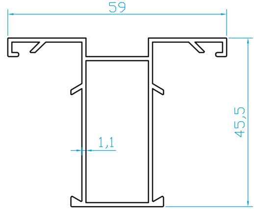
K511 DAR ALDOKS FUGALI KAYIT (0.600 Kg/m)
