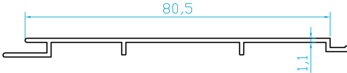
K858 YAPRAK LAMBRI (0.330 Kg/m)
