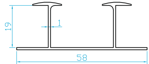
K875 MOBİLYA DEKO. PROFİL (0.325 Kg/m)
