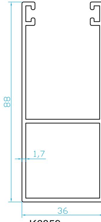
K6859 36x88 PANJUR KASA (1.205 Kg/m)
