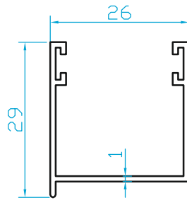
K532 FİTİLLİ PANJUR U (0.250 Kg/m)
