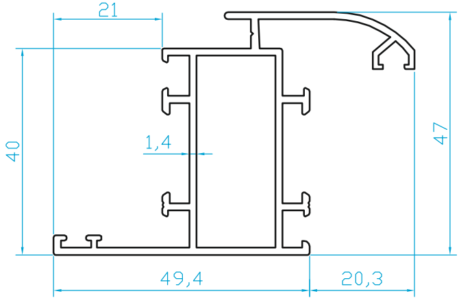
K447 DAR KANAT (0.910 Kg/m)
