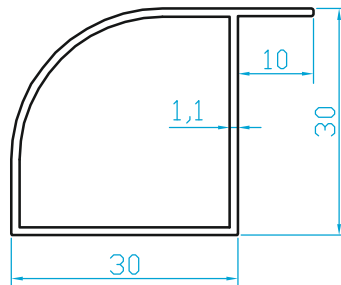
K6800 30x30 OVAL KÖŞE (0.330 Kg/m)
