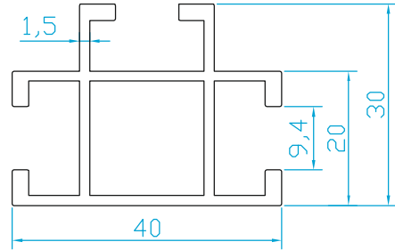
K5522 LARA VİTRİN PROFİLİ (0.690 Kg/m)
