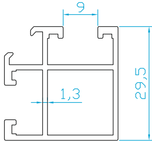
K5524 DİLARA VİTRİN (0.520 Kg/m)
