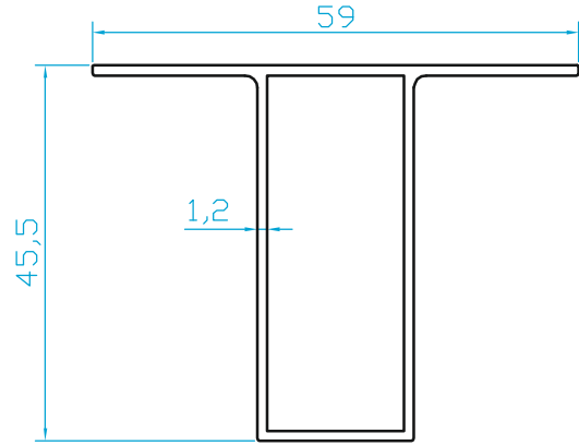
K6693 ALDOKS "T" KUTU (0.550 Kg/m)
