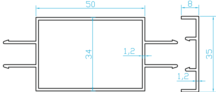
K630 JALUZİ KASA (0.800 Kg/m)
