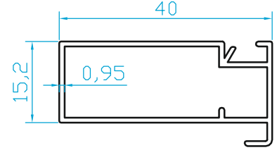
K6857 MOBİLYA PROFİLİ (0.350 Kg/m)
