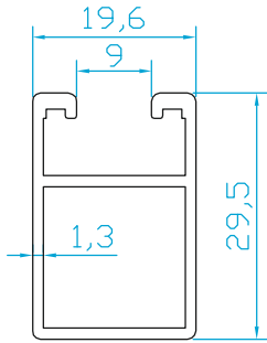
K5523 DİLARA VİTRİN (0.375 Kg/m)
