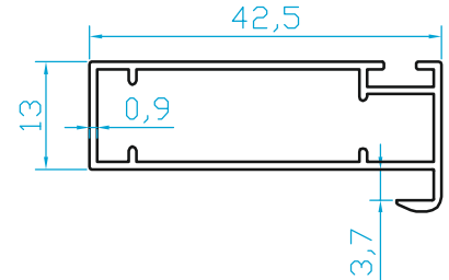
K6876 MOBİLYA PROFİLİ (0.335 Kg/m)
