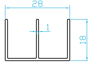
K6670 'E' PROFİL (0.215 Kg/m)
