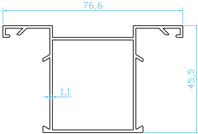
K508 GENİŞ ALDOKS FUGALI KAYIT (0.710 Kg/m)
