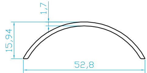
K389 OVAL KAPAK (0.285 Kg/m)
