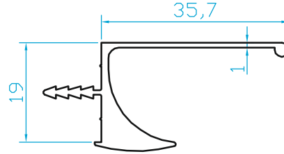
K4610 MOBİLYA PROFİLİ 0.395 Kg/m
