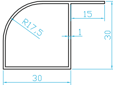
K684A 30x30 OVAL KÖŞE (0.340 Kg/m)
