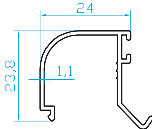
K450 ÇITA (0.250 Kg/m)
