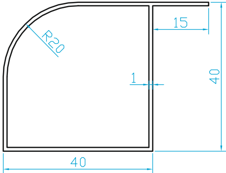
K684 40x40 OVAL KÖŞE (0.460 Kg/m)
