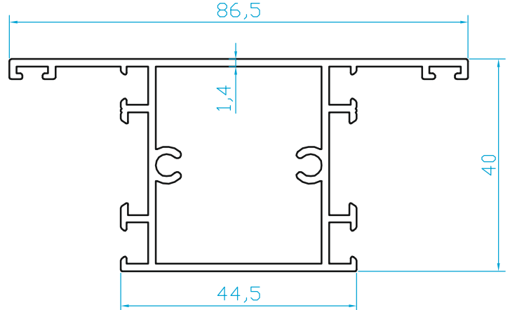
K445 KAYIT PROFİLİ (1.070 Kg/m)
