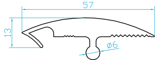
K1542 0.910 Kg/m
