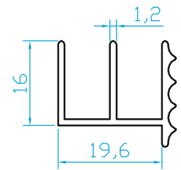
K179 'E' PROFİL (0.255 Kg/m)
