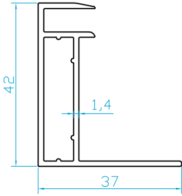
K4433 KASA PROFİLİ 0.520 Kg/m
