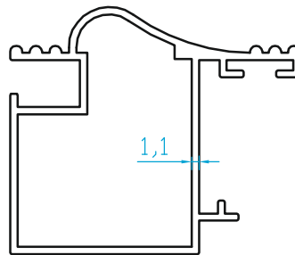
K6885 MOBİLYA PROFİLİ (0.520 Kg/m)
