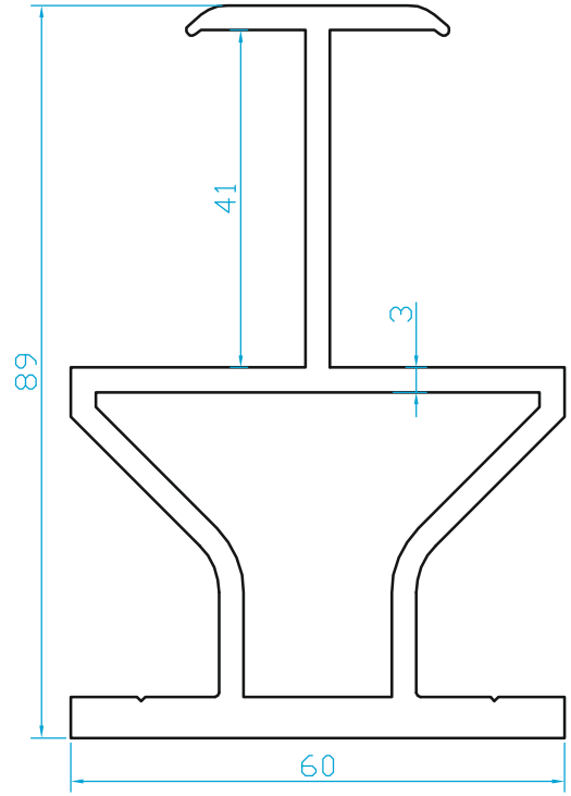
K4505 RAY PROFİLİ 2.570 Kg/m
