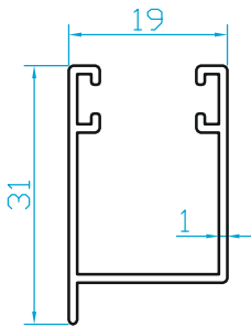
K4617 19mm FİTİLLİ U 0.245 Kg/m
