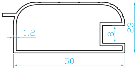
K6879 MOBİLYA PROFİLİ (0.520 Kg/m)
