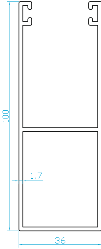
K6820 36x100 PANJUR KASA (1.320 Kg/m)
