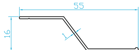
K6641 MENFEZ PANJUR (0.175 Kg/m)
