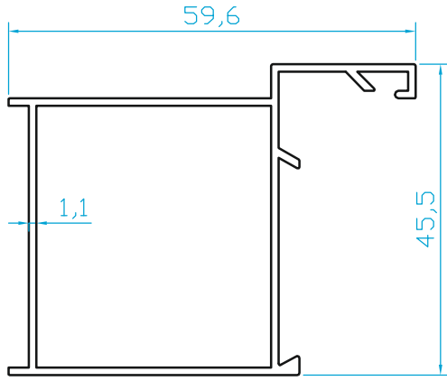
K507 GENİŞ ALDOKS FUGALI KASA (0.590 Kg/m)
