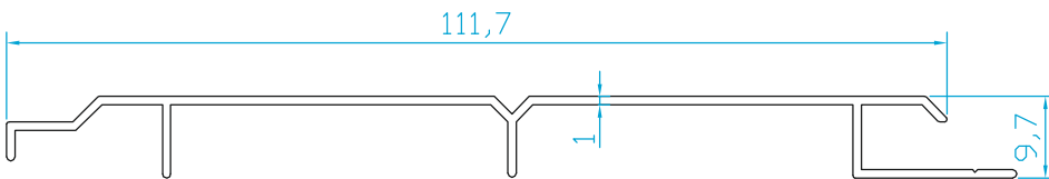
K5519 DESENLİ YAPRAK LAMBRI (0.440 Kg/m)
