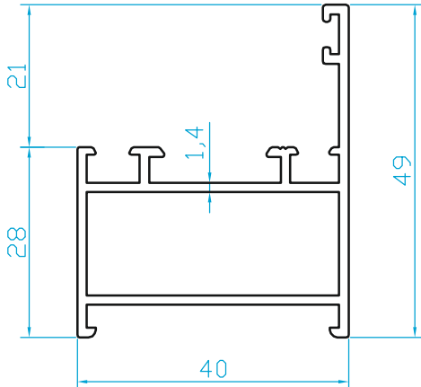
K444 KASA PROFİLİ (0.670 Kg/m)
