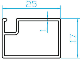
K516 SİNEKLİK (0.225 Kg/m)
