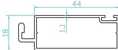
K6835 FİTİLLİ SİNEKLİK (0.460 Kg/m)
