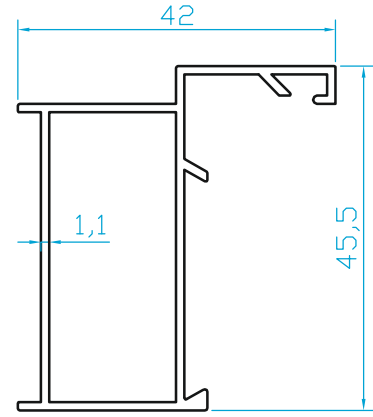
K510 DAR ALDOKS FUGALI KASA (0.490 Kg/m)
