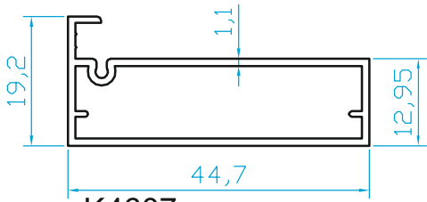
K4607 MOBİLYA PROFİLİ 0.385 Kg/m
