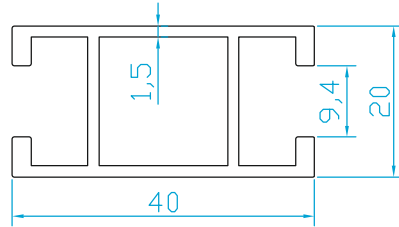
K5521 LARA VİTRİN KAYIT PROFİLİ (0.560 Kg/m)
