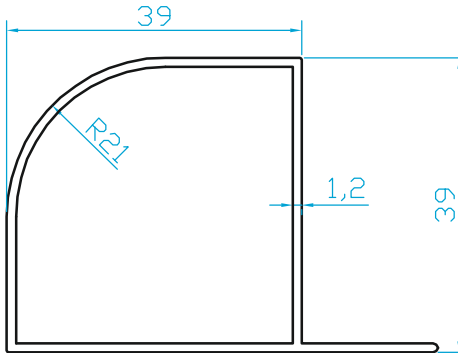
K6882 39x39 OVAL KÖŞE (0.485 Kg/m)
