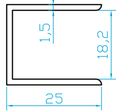
K874 ÖZEL U (0.275 Kg/m)
