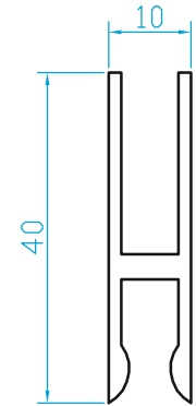
K611 'H' PROFİL (0.270 Kg/m)
