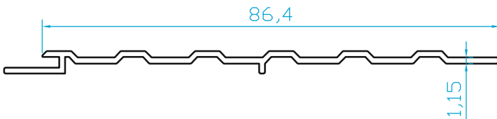
K6633 DESENLİ YAPRAK LAMBRI (0.335 Kg/m)
