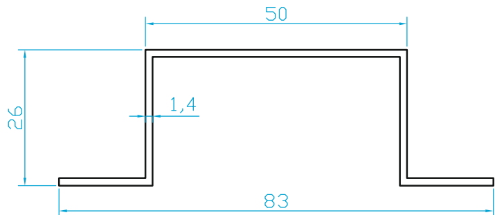
K4672 0.505 Kg/m
