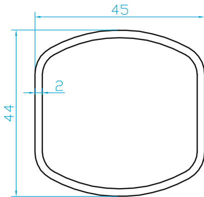
K6870 OVAL KUTU PROFİL (0.790 Kg/m)
