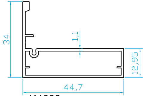
K4608 MOBİLYA PROFİLİ 0.450 Kg/m
