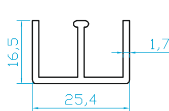
K609 'E' PROFİL (0.285 Kg/m)
