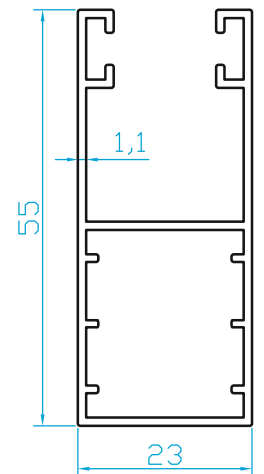
K6716 55mm PANJUR YAN "U" (0.545 Kg/m)
