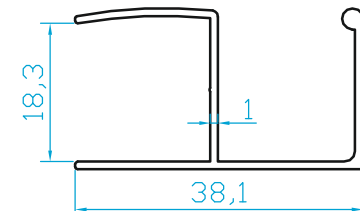
K4684 MOBİ DEKO KULP PRF. (0.280 Kg/m)
