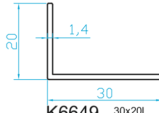
K6649 30x20L (0.190 Kg/m)
