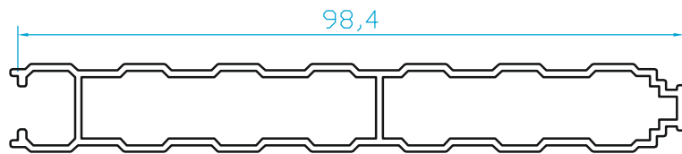
K5585 DESENLİ KUTU LAMBRI (0.660 Kg/m)
