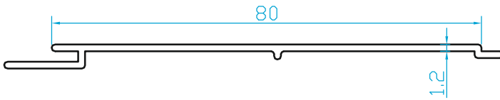
K518 YAPRAK LAMBRI (0.390 Kg/m)
