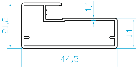
K4609 MOBİLYA PROFİLİ 0.420 Kg/m
