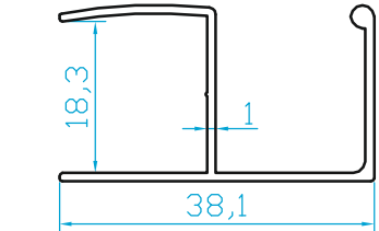
K4684 MOBİ DEKO KULP PRF. (0.275 Kg/m)
