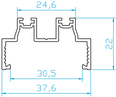
K1311 ISICAMBALKON CAM ARA PRF. (0.355 Kg/m)
