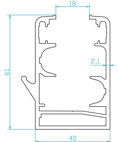
K4643 KASA (1.525 Kg/m)
