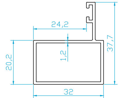
K4466 YAN KASA (0.435 Kg/m)
