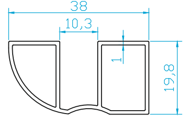
K4755 YAN BAZA (CAM) (0.360 Kg/m)
