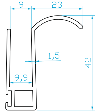
K4598 FITİLLİ CAM TUTUCU (0.500 Kg/m)
