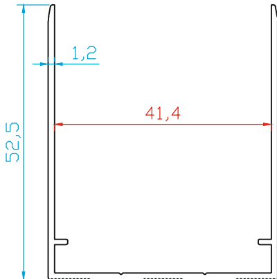
K2396 SEVİYE AYAR PROFİLİ (0.510 Kg/m)
