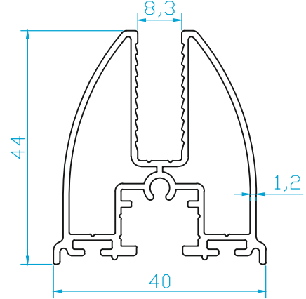
K1232 BAZA PRF.(FIRTINA) (0.785 Kg/m)
