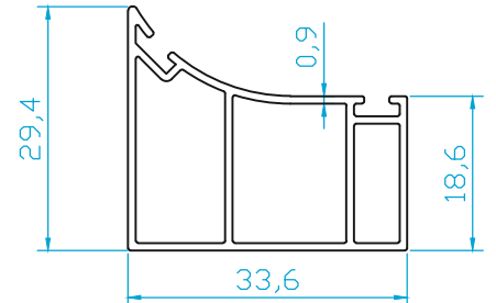
K4764 YAN BAZA (0.400 Kg/m)
