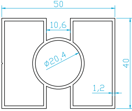
K2392 40x50 DiKME (0.850 Kg/m)
