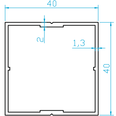
K2425 40x40 DİKME (0.615 Kg/m)
