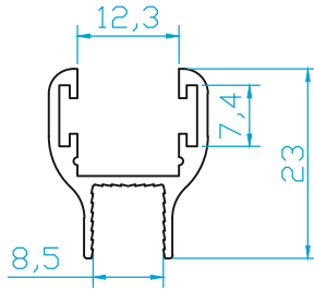
K4631 8mm CAM U (0.260 Kg/m)
