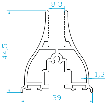
K4700 KATLANIR KANAT (0.830 Kg/m)
