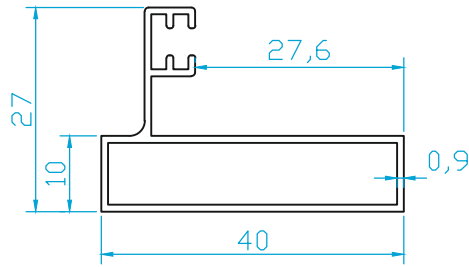
K4519 DiKME (0.325 Kg/m)
