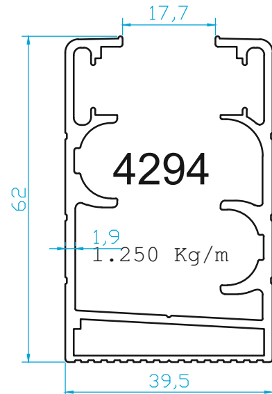
K4294 KASA PRF. 1.250 Kg/m
