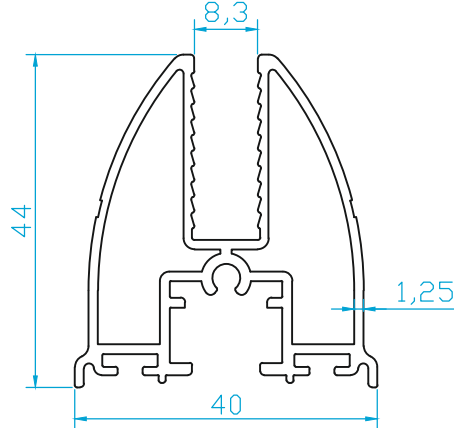
K1637 KANAT (0.870 Kg/m)
