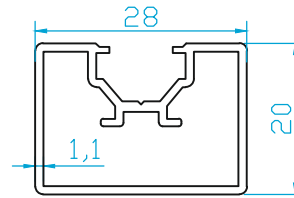
K2227 DEKOR (0.345 Kg/m)
