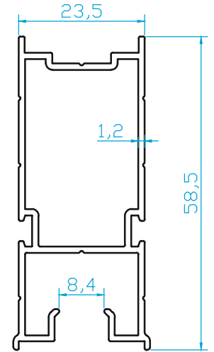
K5164 TEKCAM (8 mm) DİKME KOL PRF. 0.560 Kg/m
