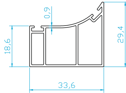
K4764 DİKME PROFİLİ (0.400 Kg/m)
