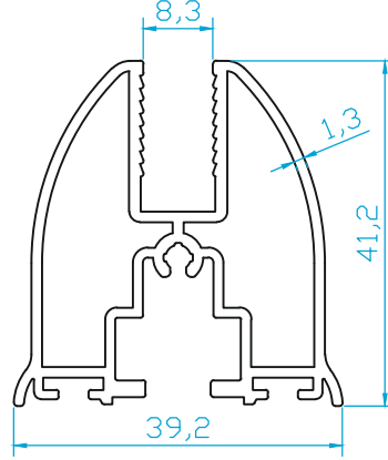
K1736 KANAT (0.830 Kg/m)
