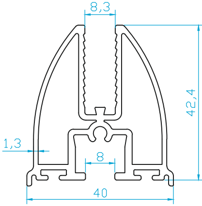
K4465 KANAT (0.985 Kg/m)
