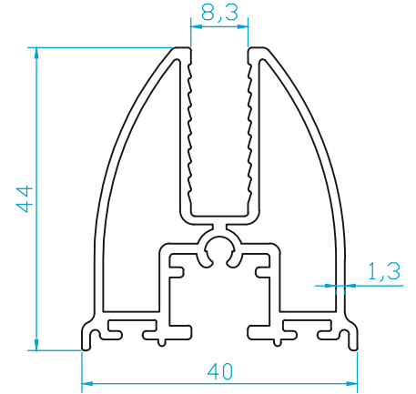
K4642 KANAT (0.910 Kg/m)
