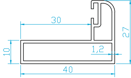
K4438 DiKME / 0.460 Kg/m
