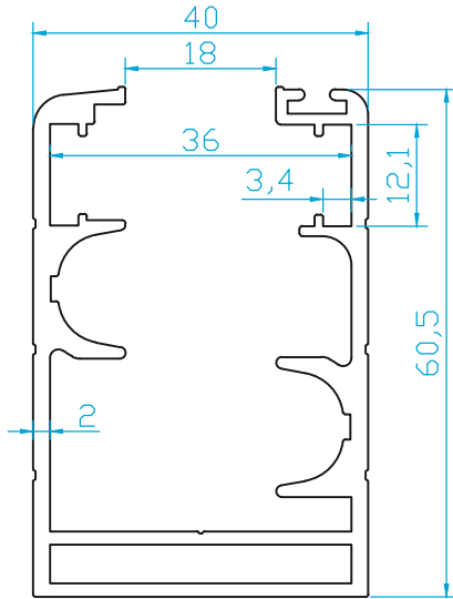
K4634 TEK FİTİL KASA (1.410 Kg/m)
