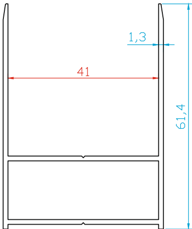
K4963 SEVİYE AYAR PROFİLİ (0.725 Kg/m)
