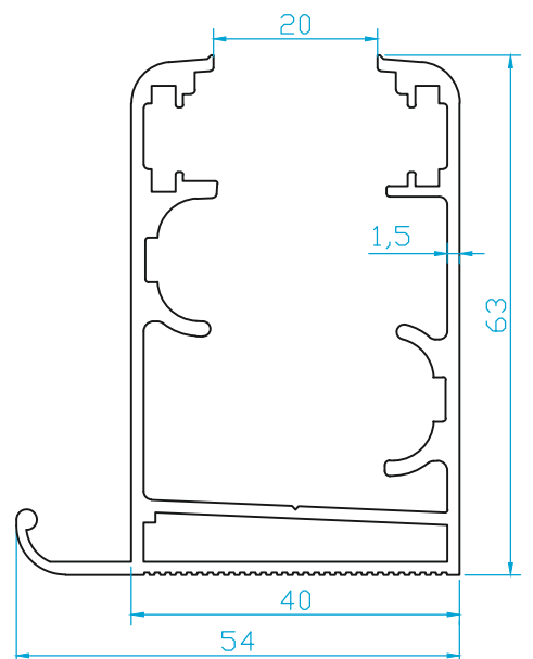
K4746 KASA (1.315 Kg/m)
