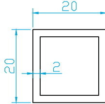
(K1501) 20X20 (0.390 Kg/m)
