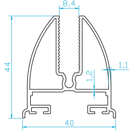
K4593 A KATLANIR KANAT (0.730 Kg/m)
