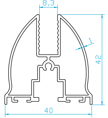
K4853 A KANAT (0.680 Kg/m)
