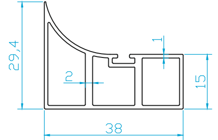
K4756 YAN BAZA (DUVAR) (0.490 Kg/m)
