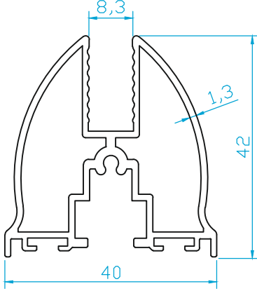
K4853 KANAT (0.785 Kg/m)
