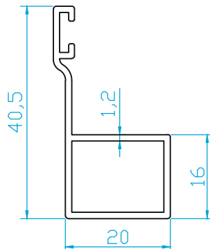
K6801 DiKME (0.335 Kg/m)
