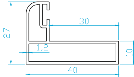
K4438 DiKME (0.460 Kg/m)
