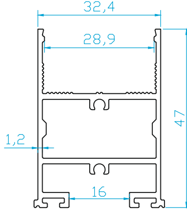
K4613 ISICAM KANAT (0.730 Kg/m)
