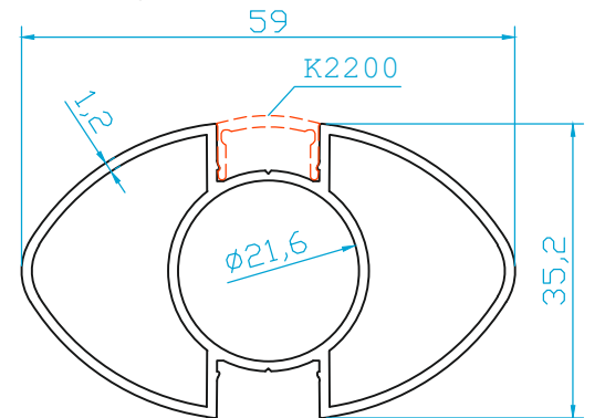
K281 OVAL DiKME (0.715 Kg/m)
