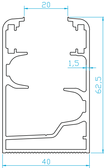
K1621 KASA (1.215 Kg/m)
