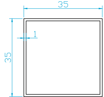
(K5550) 35X35 KUTU (0.365 Kg/m)
