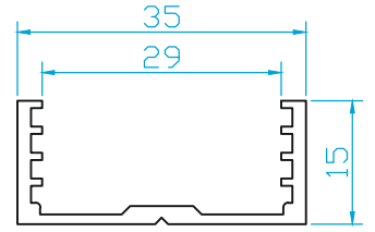
K4637 DİKEY KANAT (0.300 Kg/m)
