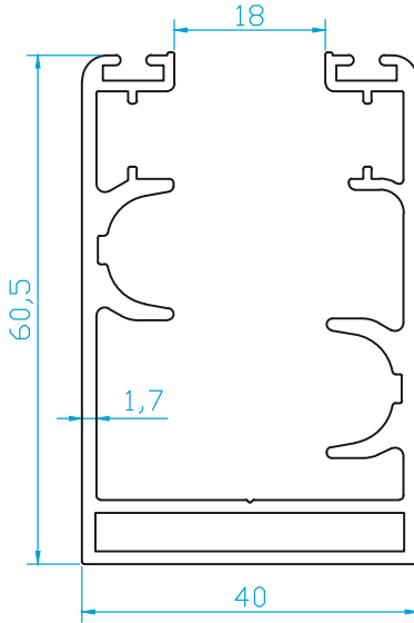
K4463 A KASA-HAFİF (1.300 Kg/m)
