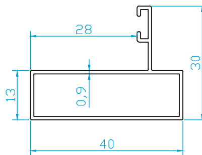
K4852 DİKME (0.325 Kg/m)
