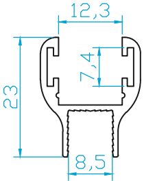
K4631 8mm CAM FİTİL 0.260 Kg/m
