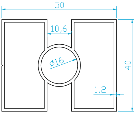
K2359 40x50 DiKME (0.930 Kg/m)
