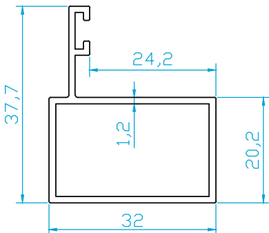
K4466 YAN KASA (0.435 Kg/m)
