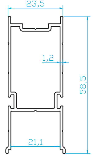
K5161 ISICAM DİKME KOL PRF. 0.560 Kg/m
