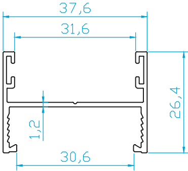
K1310 ISICAMBALKON CAM ARA PRF. (0.350 Kg/m)
