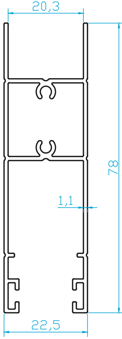
K5159 ISICAM BAZA (0.720 Kg/m)
