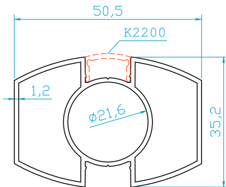
K280 YARIM OVAL DiKME (0.720 Kg/m)
