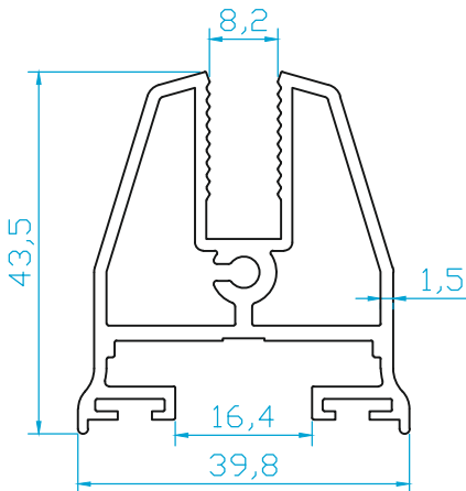
K4612 KATLANIR KANAT 0.970 Kg/m
