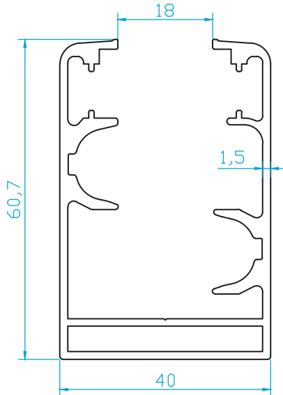
K4641 A KASA (1.230 Kg/m)
