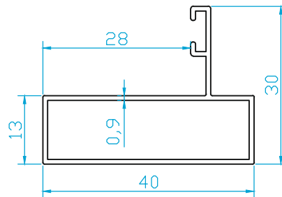
K4852 DİKME (0.325 Kg/m)
