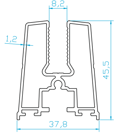
K1241 BAZA PROFİLİ 0.825 Kg/m
