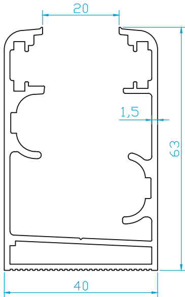
K4745 KASA (1.235 Kg/m)
