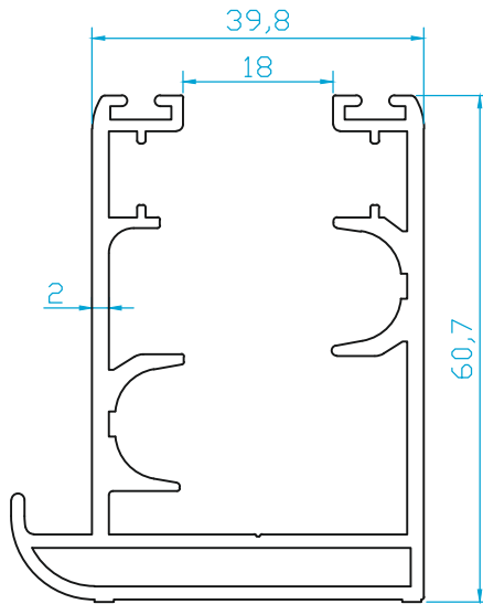
K4759 DAMLALIKLI KASA (1.450 Kg/m)
