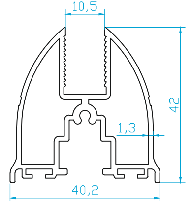
K4499 KANAT (0.820 Kg/m)
