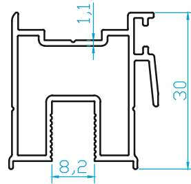
K5163 TEKCAM (8 mm) KENET 0.440 Kg/m
