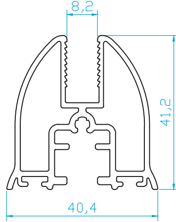
K4630 KANAT (0.925 Kg/m)
