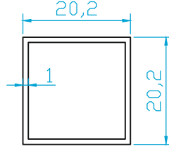
(K6868) 20.2x20.2 (0.210 Kg/m)
