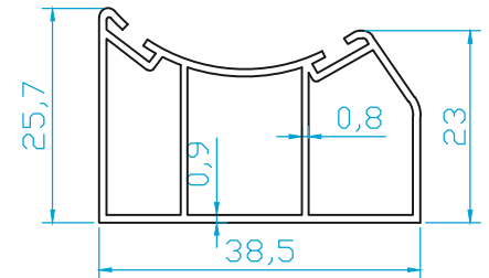
K4723 YAN BAZA (0.410 Kg/m)
