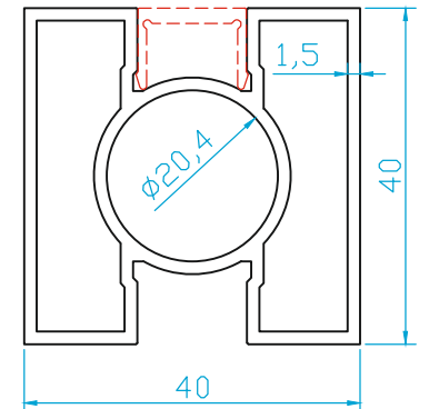
K252 KARE DİKME (0.960 Kg/m)
