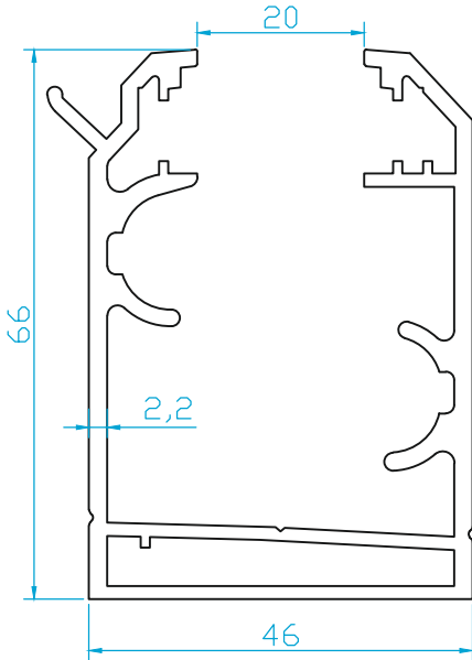
K4885 ISICAMLI KASA 1.620 Kg/m
