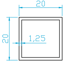
(K1501) 20X20 (0.255 Kg/m)
