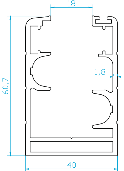
K4634 TEK FİTİL KASA (1.410 Kg/m)
