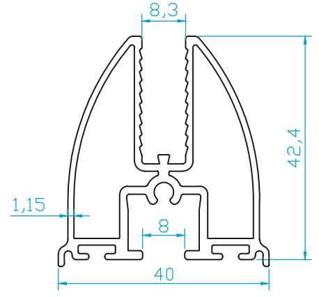
K4465 B KANAT-HAFİF (0.860 Kg/m)
