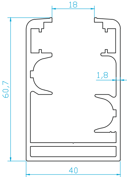
K4641 KASA (1.411 Kg/m)
