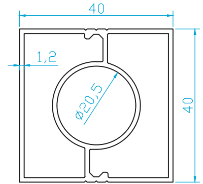
K2365 40x40 DİKME 0.810 Kg/m
