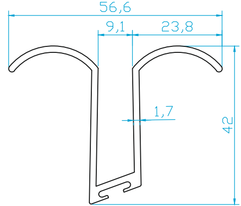
K4552 FITİLLİ CAM TUTUCU (0.625 Kg/m)
