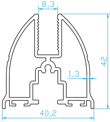
K4459 KANAT (0.845 Kg/m)
