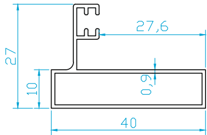
K4519 DiKME (0.325 Kg/m)
