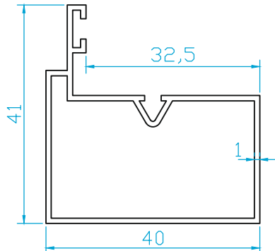
K4483 YAN KASA (0.440 Kg/m)
