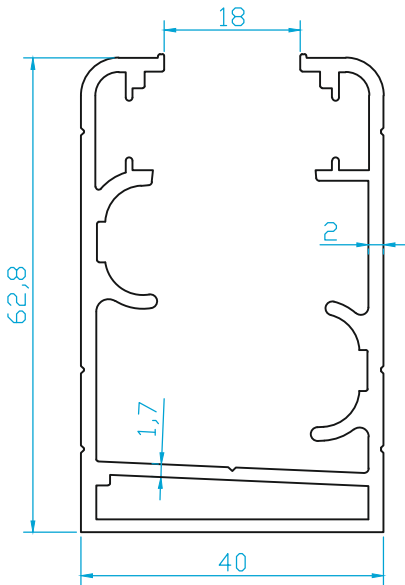
K4854 KASA (1.375 Kg/m)
