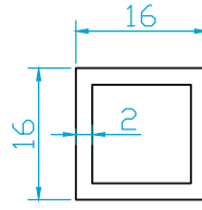
(K4527) 16X16 (0.300 Kg/m)
