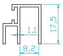
K4494 CAM TUTUCU 8mm 0.190 Kg/m
