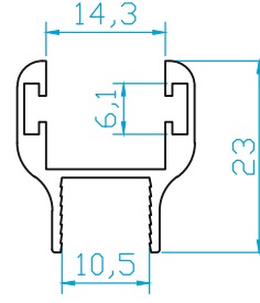
K4479 10 mm CAM FİTİL 0.275 Kg/m
