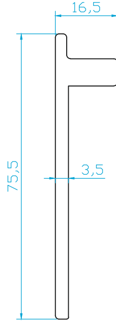
K1511 CAM AYAR PROFİLİ 0.960 Kg/m
