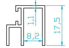
K4494 CAM TUTUCU 8 mm 0.190 Kg/m
