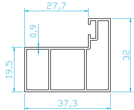
K1664 YAN DİKME (0.440 Kg/m)
