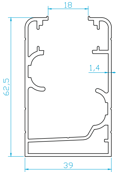
K4854 B (SVS) KASA (1.090 Kg/m)
