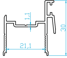
K5160 ISICAM KENET 0.295 Kg/m
