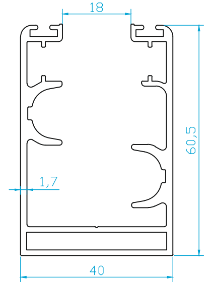
K4463 A KASA-HAFİF 1.300 Kg/m
