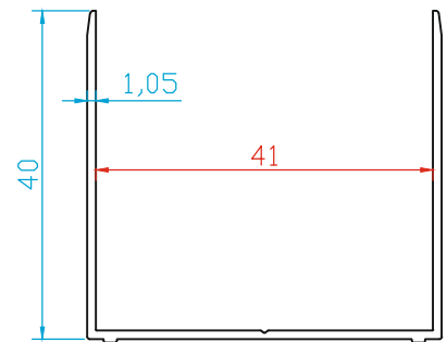
K1920 SEVİYE AYAR PROFİLİ (0.350 Kg/m)
