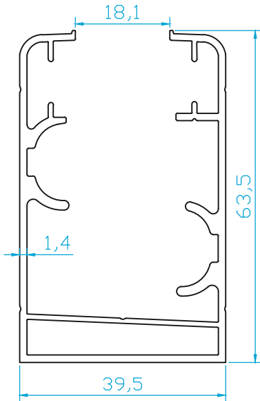
K4261 CAMBALKON KASA 1.060 Kg/m
