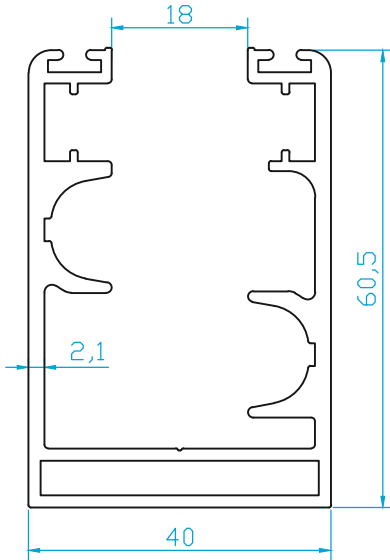
K4463 KASA (1.440 Kg/m)
