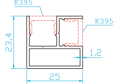
K1665 CAM TUTUCU (0.335 Kg/m)
