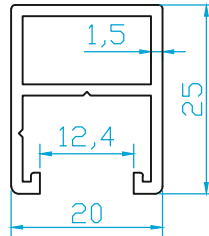
K2249 CAM KENAR 0.370 Kg/m
