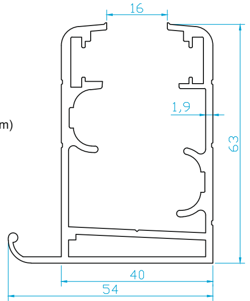
K4430 KASA (1.510 Kg/m)
