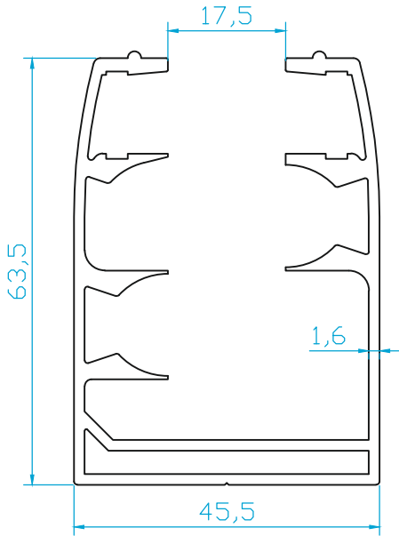
K4620 CAM BALKON KASA (1.465 Kg/m)
