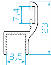
K4632 8mm CAM FİTİL 0.170 Kg/m
