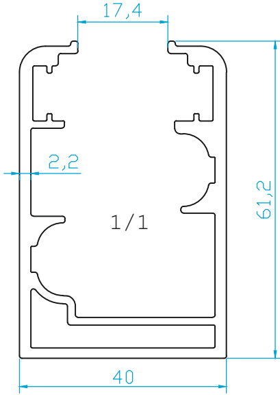
K4629 KASA (1.460 Kg/m)
