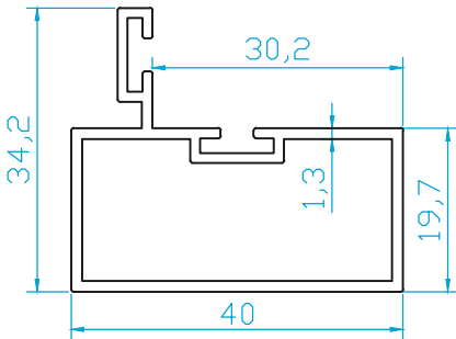
K4661 DiKME (0.520 Kg/m)
