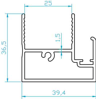
K5362 BAZA JALUZİ CAM (0.690 Kg/m)
