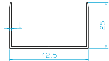
K4484 YAN KASA U PRF. (0.245 Kg/m)
