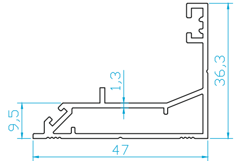
K4615 YAN DİKME 0.550 Kg/m
