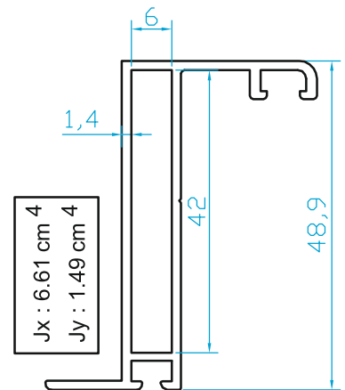
K4588 ALUNEW SERİ GİZLİ KANAT KASA PRF (0.585 Kg/m)
