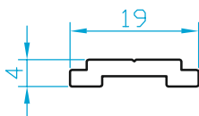
K817 TİJ (0.150 Kg/m)
