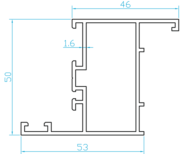
K802 C50 DAR NORMAL KASA (1.165 Kg/m)
