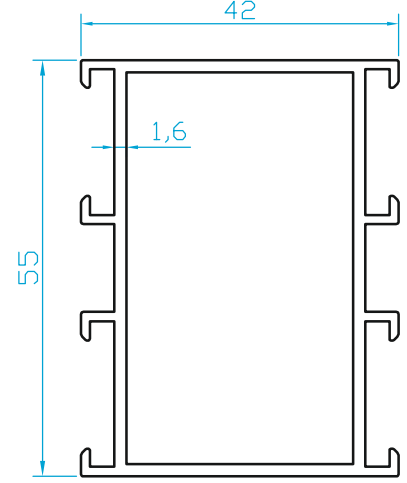
K410 KASA (0.960 Kg/m)
