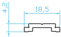
K962 TiJ PROFİLİ (0.125 Kg/m)
