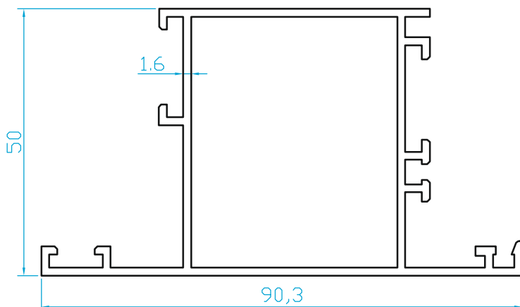
K801 C50 GENİŞ ORTA (1.135 Kg/m)
