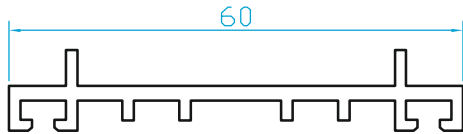
K820 TIRNAKLI KASA İLAVESİ (0.475 Kg/m)
