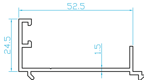
K809 İLAVE PROFİLİ (0.400 Kg/m)
