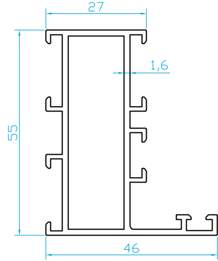
K432 DAR KASA (0.920 Kg/m)
