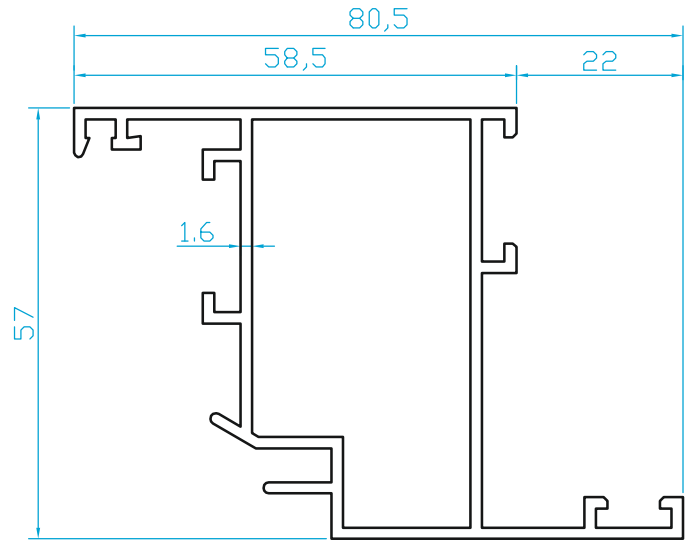
K804 C50 GENİŞ KANAT (1.150 Kg/m)
