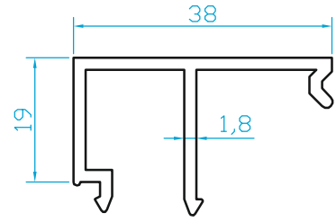
K2919 TEKCAM ÇİTASI (t:1.3 mm = 0.330 Kg/m) (t:1.8 mm = 0.420 Kg/m)
