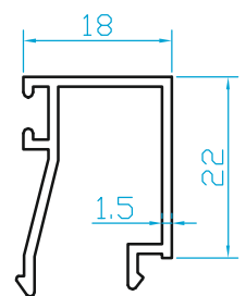
K816 FİTİLLİ CAM ÇİTASI (0.255 Kg/m)
