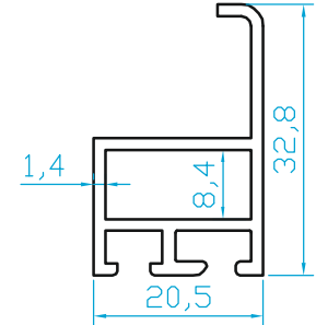
K4586 ALUNEW SERİ CAM KASET PRF. (0.396 Kg/m)
