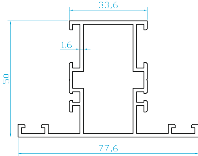
K800 C50 DAR ORTA (1.106 Kg/m)
