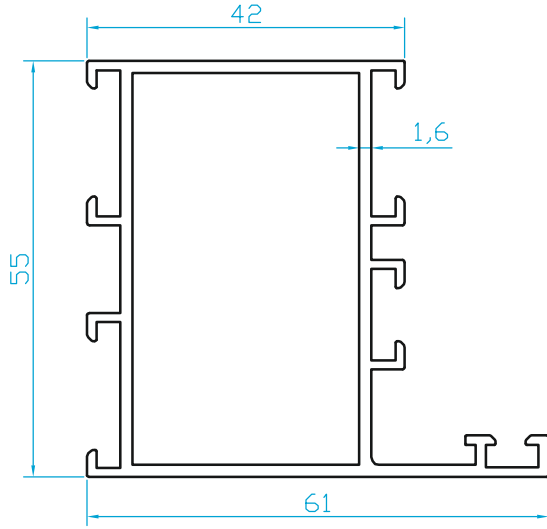
K402 GENİŞ KASA (1.100 Kg/m)
