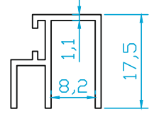
K4494 CAM TUTUCU 8 mm 0.190 Kg/m
