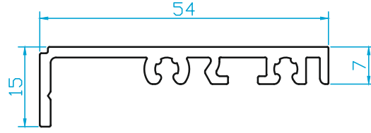
K5756 LINEER MOTOR CASE COVER (Bioclimatic Pergola System ) 0.545 Kg/m
