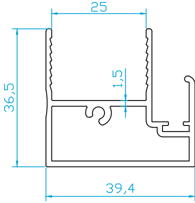
K5362 BAZA JALUZİ CAM (0.690 Kg/m)
