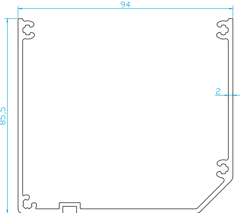
K5758 MOTOR CASE PROFİLE (Bioclimatic Pergola System ) 1.620 Kg/m
