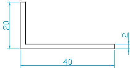
K1350 40x20 Winkel 0.315 Kg/m
