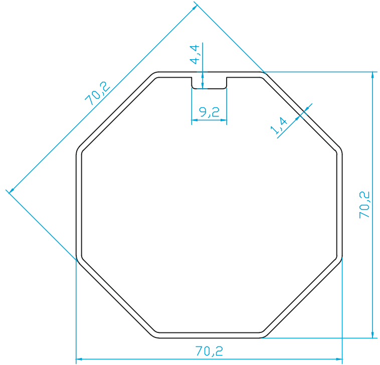
K5499 TENTE & GİYOTİN MOTOR PROFİLİ (0.990 Kg/m)
