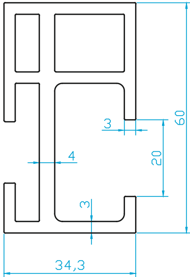
K5757 SMALL RAİL PROFİLE (Bioclimatic Pergola System ) 1.950 Kg/m
