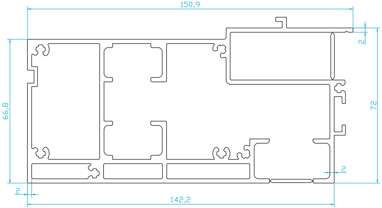
K5759 RAİL PROFİLE (Bioclimatic Pergola System ) 4.660 Kg/m
