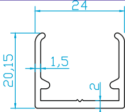
K1339 Abdecker klick 0.310 Kg/m
