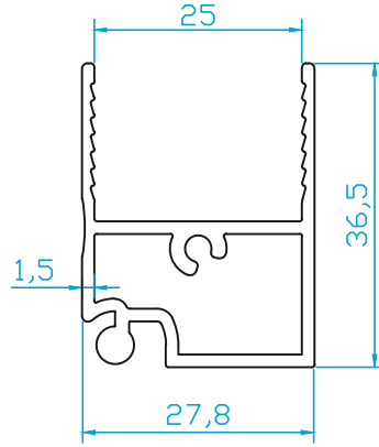
K5363 SABİT BAZA JALUZİ CAM (0.570 Kg/m)
